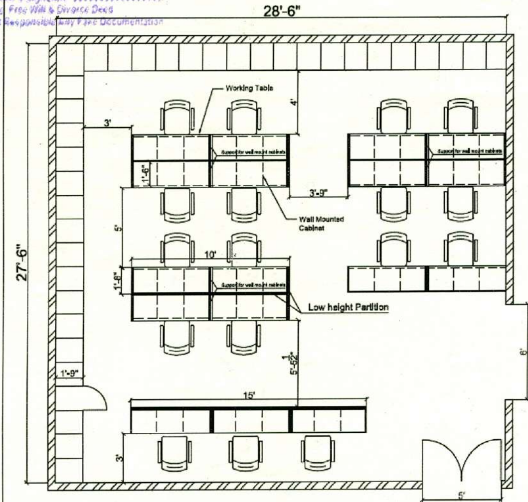
FURNITURE LAYOUT OF EXAMINATION DEPARTMENT (CITY CAMPUS)
