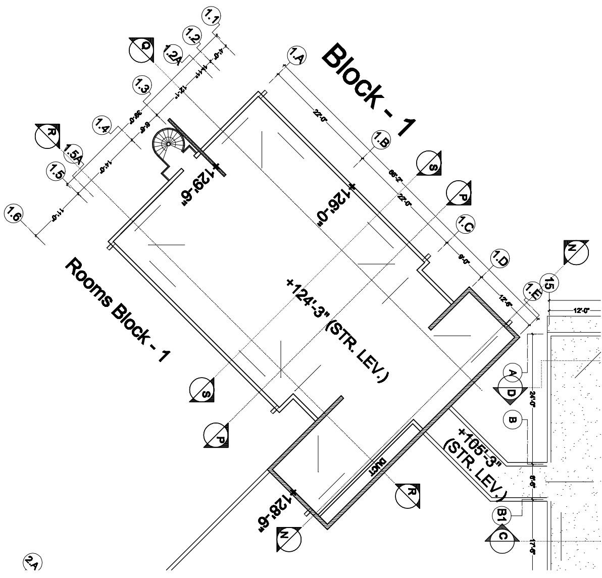
Roof Plan
