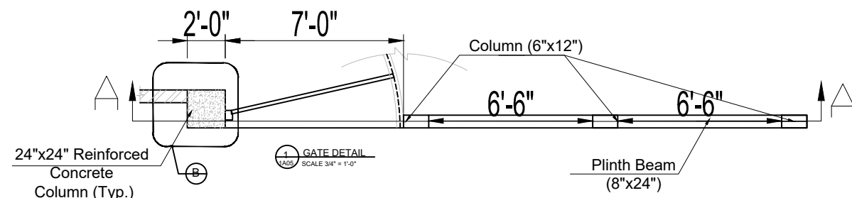
SITE PLAN
