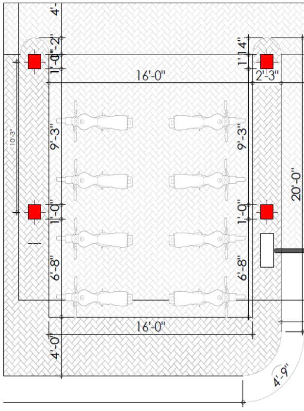
09 MOTORCYCLE STALL PLAN Scale: 1/4" = 1'-0"
