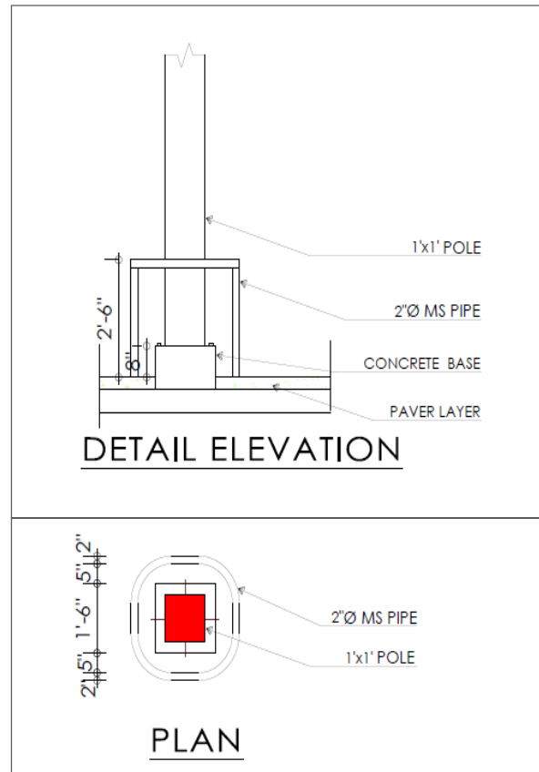
10 COLUMN PROTECTION DETAIL Scale: 1/4" = 1'-0"
