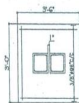
DOUBLE COL. FOOTING
