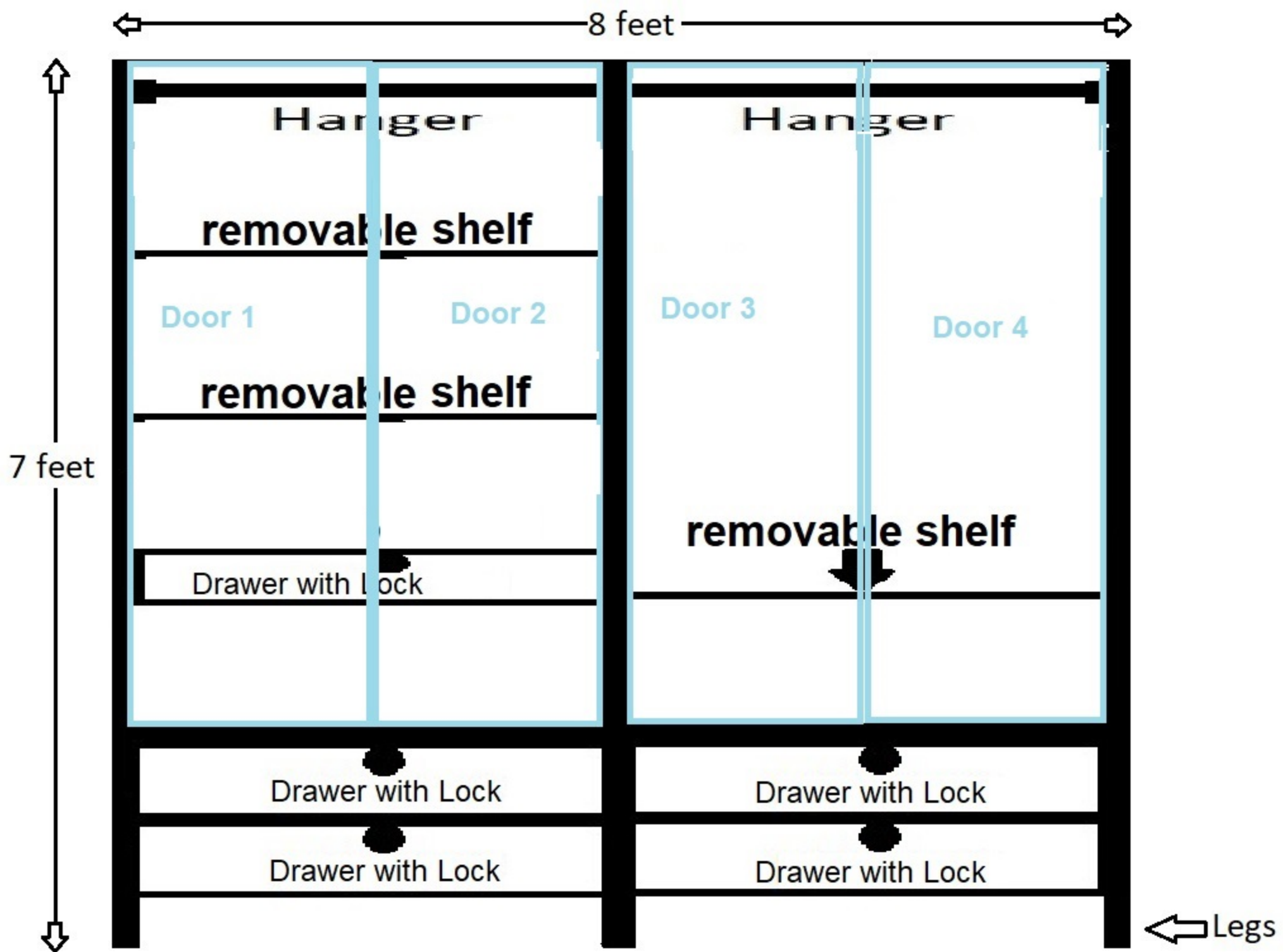
Inside view of four cabinets
