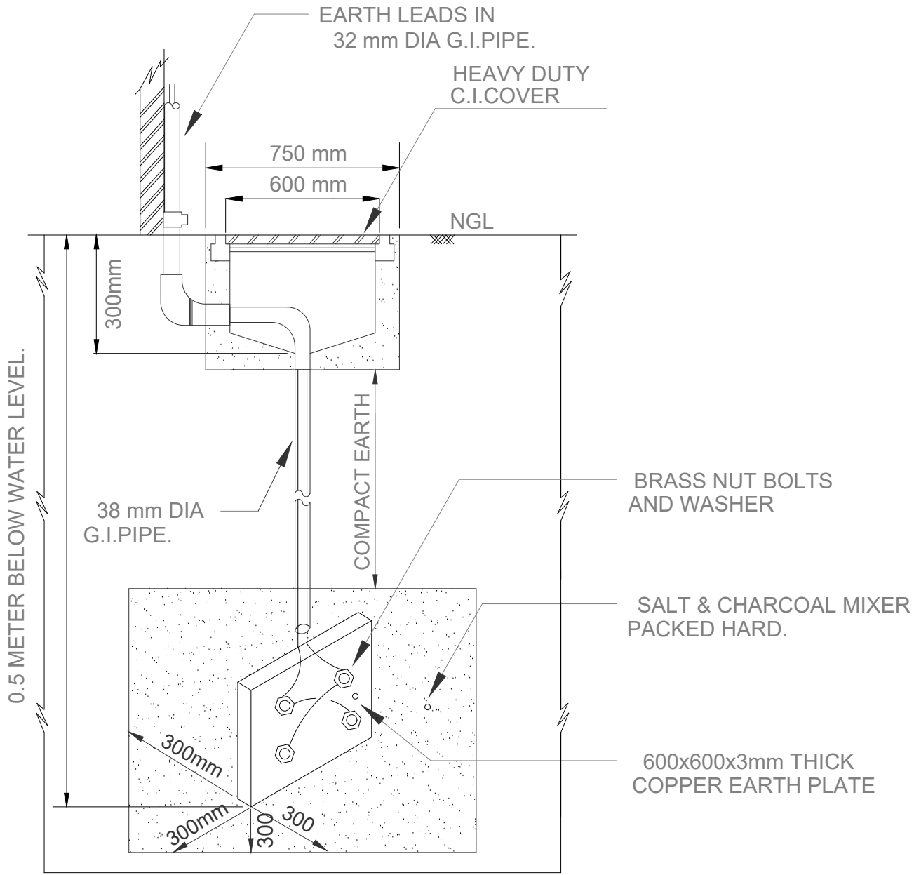
EARTHING DETAIL
