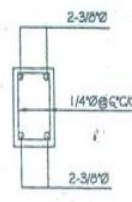
DETAIL "C" BEAM 6" X 12"
