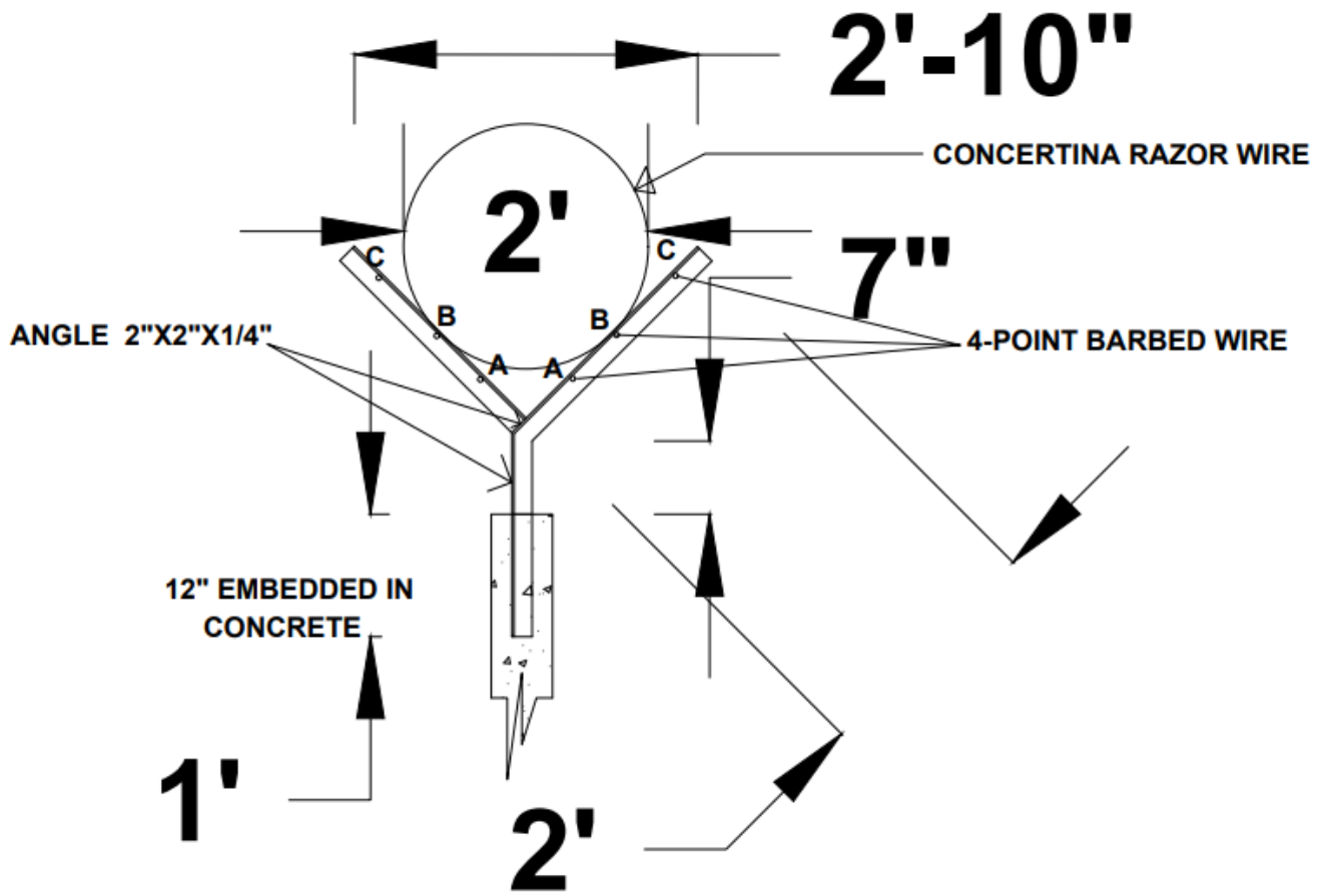
TYPICAL ARRANGEMENT OF Y-POST CONCERTINA RAZOR WIRE 24" DIA AND BARBED WIRE
